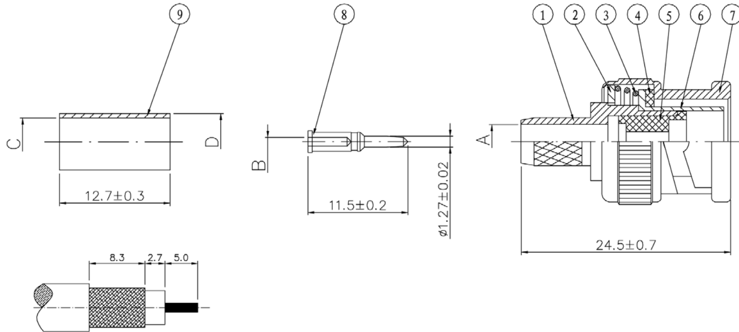
RECOMMENDED CABLE STRIPPING DIM'S
